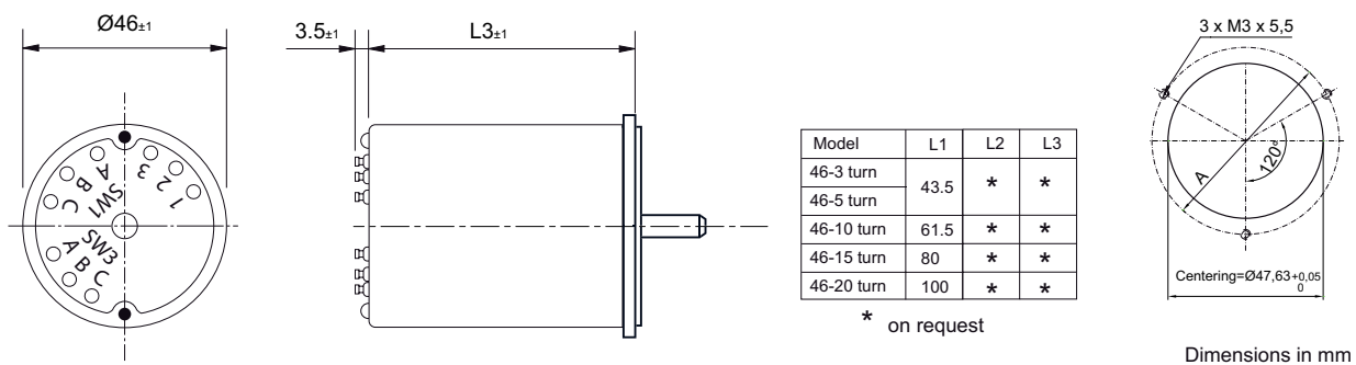
Version with limit switch
