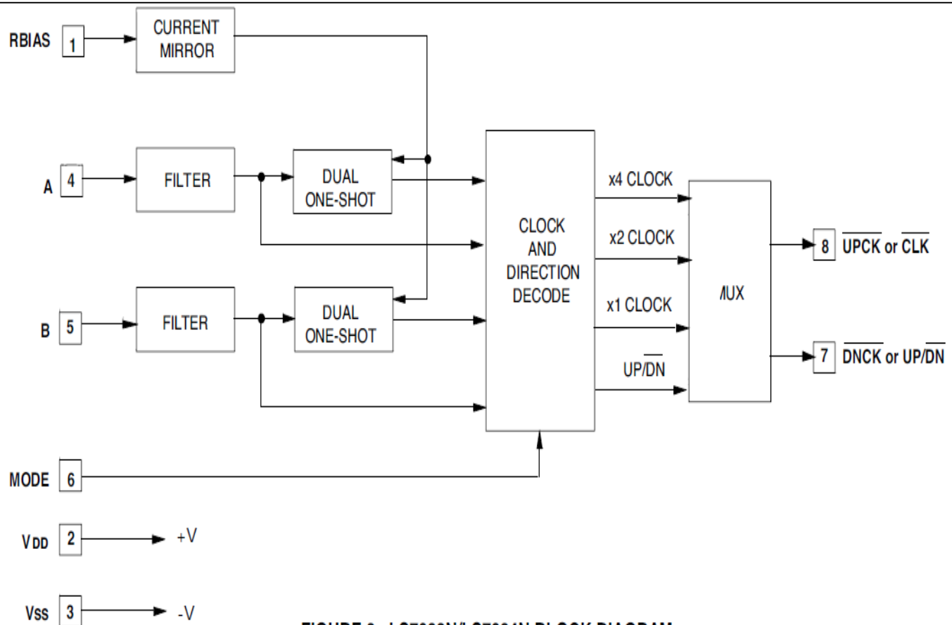
FIGURE 3. LS7083N/LS7084N BLOCK DIAGRAM
